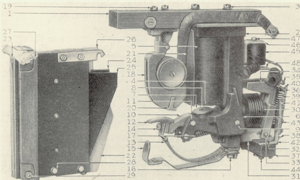
TYPE DB-984 FORM A LINE BREAKER
